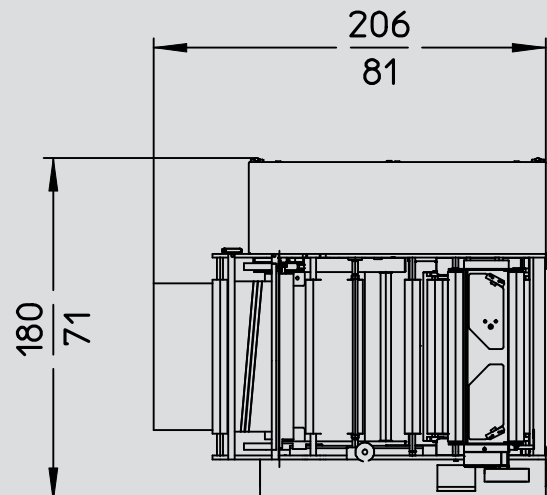
Floorplan UW52-770
