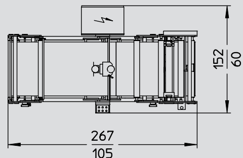
Floorplan PFS
